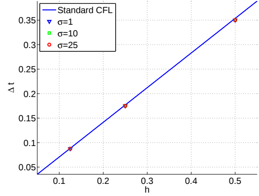
Figure 2: CFL condition for scheme B with a Q_1 - Q_1^{\text{disc}} discretization and a constant absorbing function.
