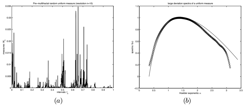
Figure 2: (a): one realization of a uniform random measure W (resolution n = 10 ); (b): theoretical spectrum and estimation result for this realization.
