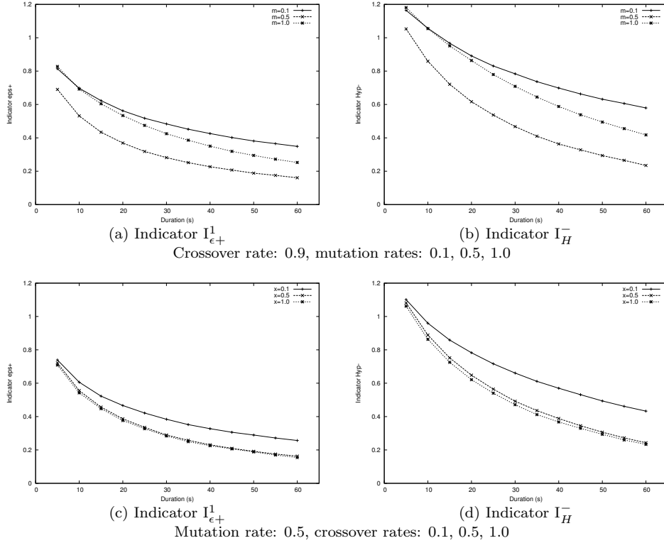
Figure 6: Average evolution of the quality of solutions of 10 realistic instances over 20 runs (1 minute per instance, NSGA-II used) according to three crossover and three mutation rates.
