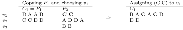
Figure 3: Example of crossover of two solutions P_1, P_2 for producing a new individual C_1 .
