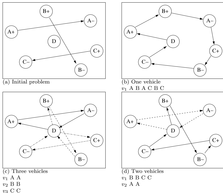
Figure 1: Examples of solution encoding: (a) Initial problem with three customers A, B, C, (b) a solution with one vehicle (one route), (c) a solution with three vehicles (three routes), (d) a solution with two vehicles (two routes).
