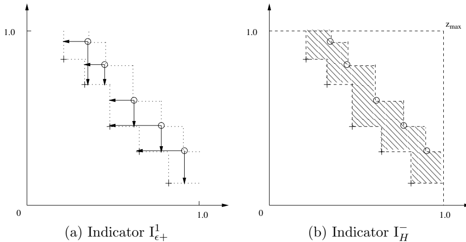
Figure 5: Comparison of the quality of Pareto solution sets according two indicators: I_{c+}^1 and Indicator I_H^- in the objective space (approximation set 'o' is compared with reference set '+')
