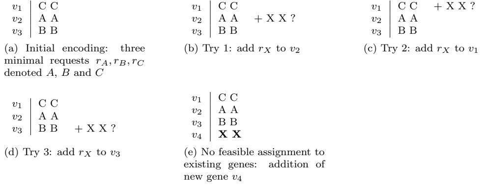
Figure 2: Example of initialization with four requests: r_A, r_B, r_C, r_X . \{r_A, r_B, r_C\} \in R_{min}
