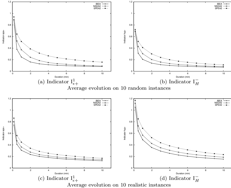
Figure 7: Average evolution of quality of solutions on 10 realistic and 10 random instances over 20 runs (100 requests per instance, 10 minutes per run , mutation: 0.5, crossover: 0.9).
