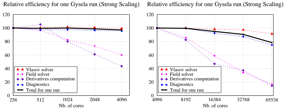
Figure 5: Small case, GYSELA efficiency Figure 6: Big case, GYSELA efficiency
