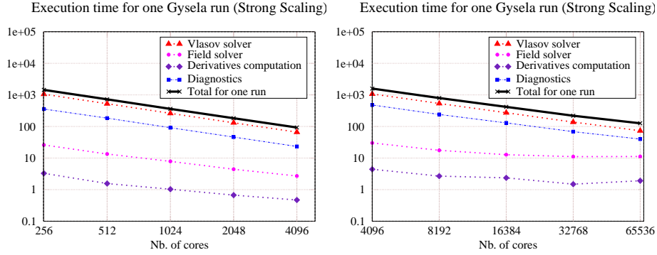
Figure 3: Small case - GYSELA timings Figure 4: Big case - GYSELA timings
