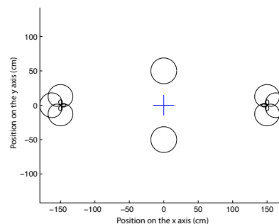
Fig. 2: Microphone array configuration of the side-ICLD microphone array.
