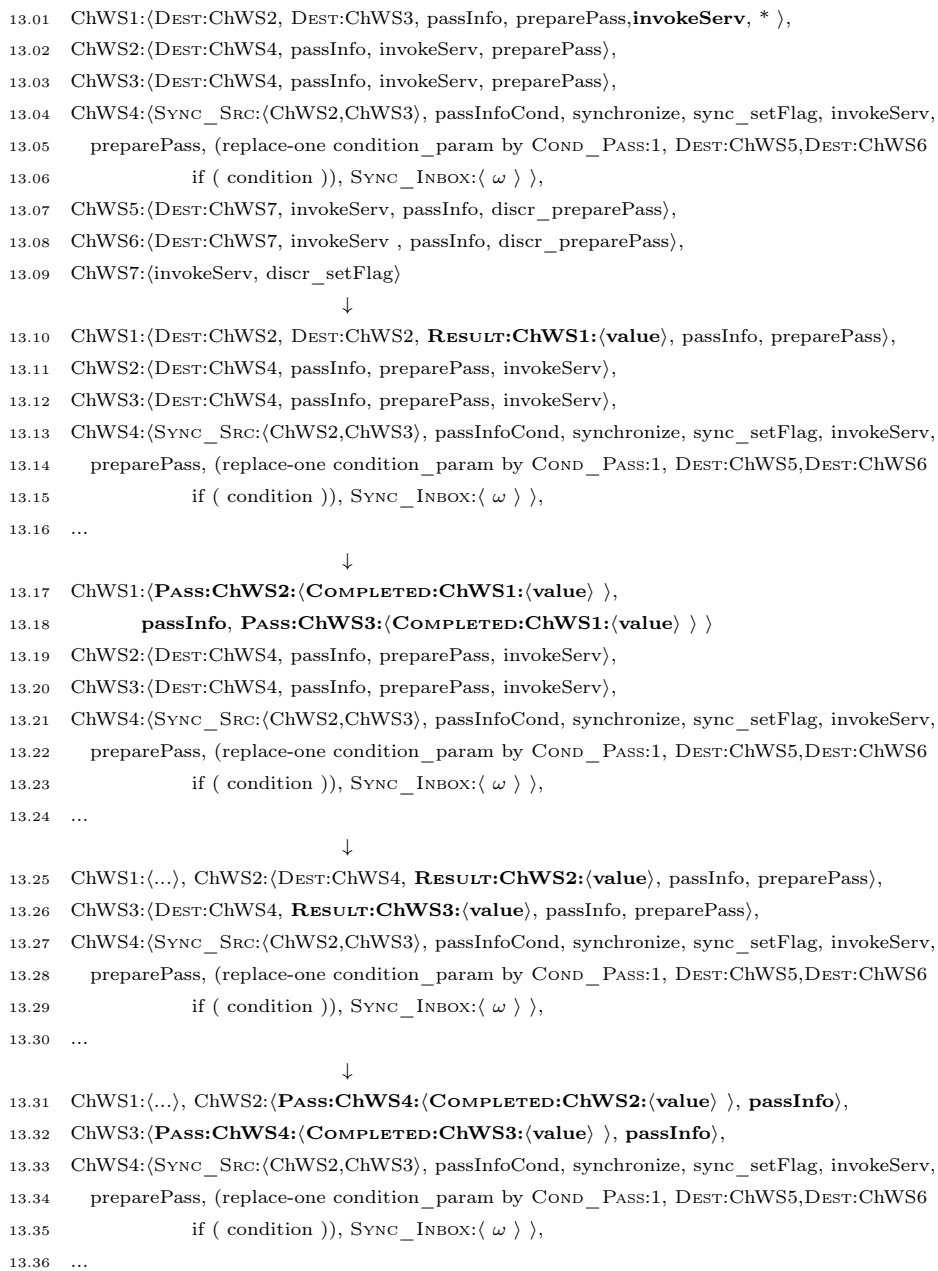
Figure 15: Workflow execution, steps 0-4.
