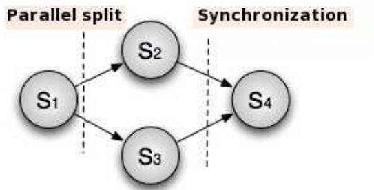
Figure 4: Simple workflow example.
