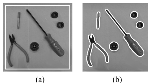
Fig. 11. (a) Image along with initial contour. (b) The converged contours.
