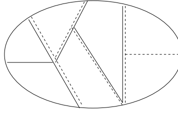
Figure 6. Example of partitions like \Pi_1 (solid line) and \Pi_2 (dashed line) in Theorem 13.
