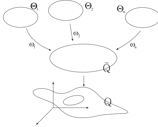
Figure 5. Families of feature spaces involved in the object tracking problem. The actual continuous parameter space \mathcal{Q} of the articulated object is unknown, while its finite approximation \tilde{\mathcal{Q}} is the common refinement where the evidence extracted from the image is combined.
