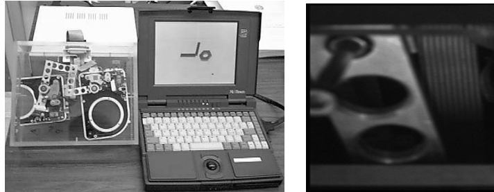
Figure 4. The PantoMouse planar robot (left). Its pose is just the 2D position of its end-effector (right).
