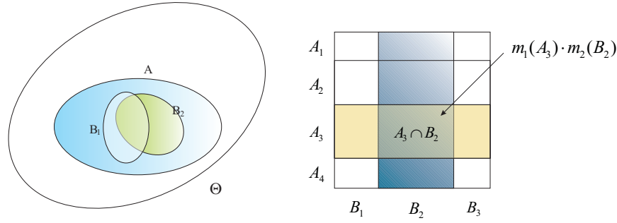
Figure 1. Left: Basic probability assignment and belief value. In the picture m(B) \neq 0, B \subset A only for B_1 and B_2 so that s(A) = m(B_1) + m(B_2) . Right: Dempster's rule of combination: on the y,x axes are depicted the focal elements A_i and B_j of s_1, s_2 respectively. The width of columns and rows is proportional to the b.p.a. associated with each focal element (in a size 1 square). Each intersection is given the product of the corresponding masses (equal to the area of the related square). Contributions of coincident intersections are then summed. This value is finally normalized by taking into account all the empty intersections (denominator of Equation (2)).
