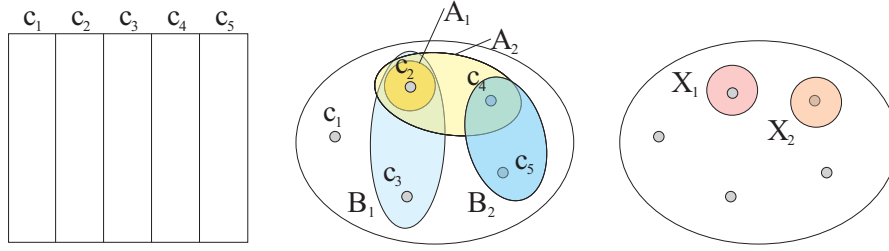
Figure 2. The frame (middle) associated with a partition of the column range of an image (left). The b.f. s_1 with focal elements A_1, A_2 and s_2 with f.e. B_1, B_2 (middle) can be combined through Dempster's rule yielding a new belief function s_1 \oplus s_2 (right) with f.e. X_1 and X_2 .
