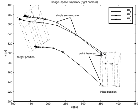
Figure 2: Initial and target image of the gripper and the feature trajectories over the iterations of the control loop.
