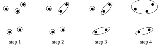
Figure 2: Hierarchical clustering algorithm
