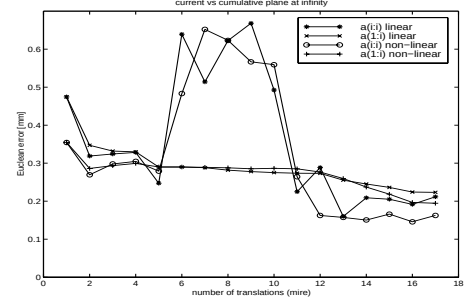
Figure 3: Comparison of single and cumulative estimates from linear and non-linear \mathbf{H}_T .
