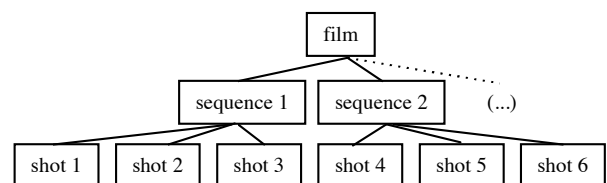
figure 2: hierarchical structure
