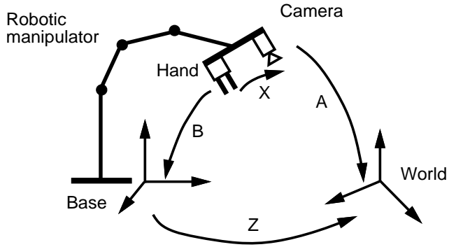
Fig. 1. Robot/world ( \mathbf{Z} ) and hand/eye ( \mathbf{X} ) calibration. The camera is mounted onto the gripper and camera motions are determined using a calibration pattern. The world frame is the frame of the calibration pattern.
