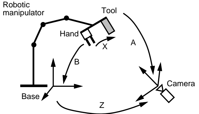
Fig. 1. Robot/world ( \mathbf{Z} ) and hand/eye ( \mathbf{X} ) calibration. The camera is mounted onto the gripper and camera motions are determined using a calibration pattern. The world frame is the frame of the calibration pattern.
