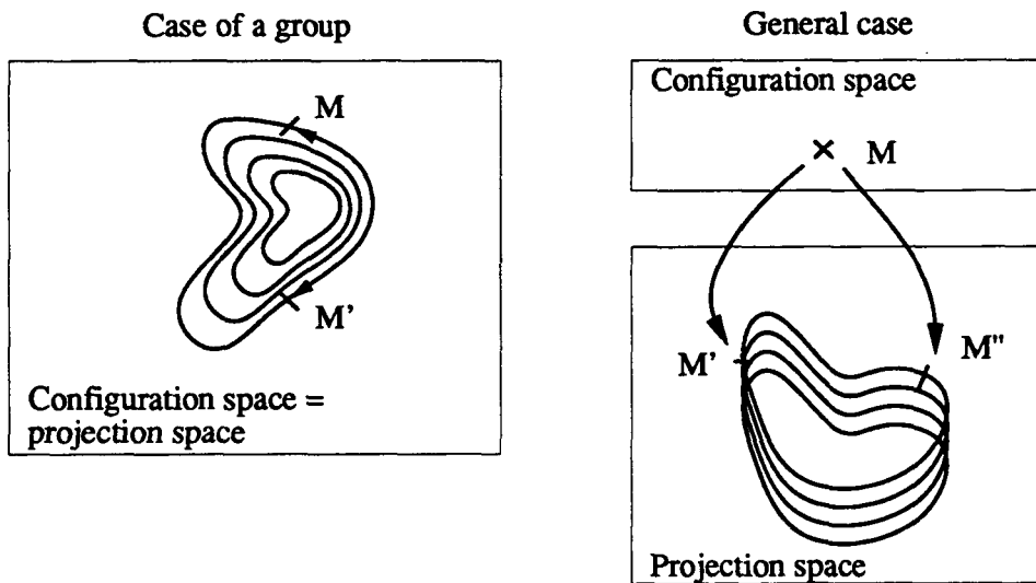
Figure 5: One orbit in the case of groups and in the general case
