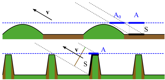
Fig. 7. Parallax offset and Jacobian. Top: for a correct rendering the surface maps must not be evaluated in A_0 , the pixel footprint on the coarse mesh ( dotted blue line ), but in the orthogonal projection A of the pixel footprint S on the complex surface (here using A_0 would give a green color, instead of brown, the correct result). Bottom: the parallax Jacobian \frac{\partial v}{\partial ng} has important effects with near vertical facets. Here without it we find the green part as dominant, in A , while in fact, orthogonally to v , this is the brown part.
