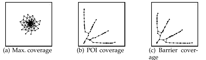
Fig. 7. Resulting graph at the end of the simulation for different coverage schemes with message loss probability \pi = 0.5 . In this simulation there is 50 nodes with a range of 10 on a square of 100 \times 100 .
