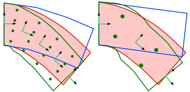
Fig. 10. Comparison of FEM simulation (in blue) and frame-based simulation (in green) for 4 \times 4 \times 4 (left) and 2 \times 2 \times 2 (right) FEM nodes and integration points. The reference high-resolution FEM is shown in red. The integration points are shown as disks. The green curve is the outline of a visual model bound to the frames.
