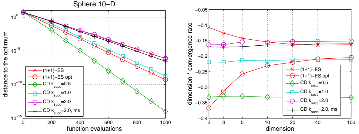
Figure 3: Left: Evolution of distance to the optimum versus number of function evaluations for the (1+1)-ES, (1+1)-ES opt, CD k_{succ}=0.5 , CD k_{succ}=1.0 , CD k_{succ}=2.0 and CD k_{succ}=2.0 ms on f(x) = \|x\|^2 in dimension 10. Right: Convergence rate c (the lower the better) multiplied by the dimension d for different algorithms depending on the dimension d . The convergence rates have been estimated for the median of 101 runs.
