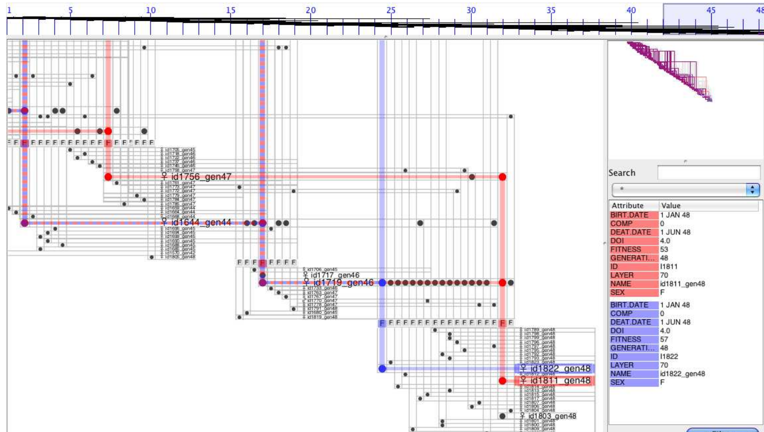
Figure 11: Rosenbrock function in dimension 10 (50 individuals during 50 generations). Track of the common ancestors of two individuals: continuous red and blue lines until the first common ancestor from which the lineage is identified with a red-blue dotted line). A filtering has been applied, to magnify the selected lineages.
