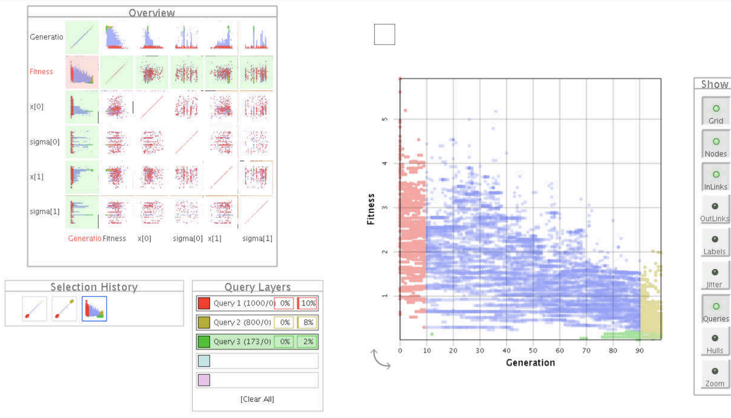
Figure 3: 2D Weierstrass function of Hölder exponent 0.2. Scatterplot and Fitness versus generation view. Red points correspond to the first 10 generations, yellow points, to the 10 last ones, and green points, to the best fitness areas.
