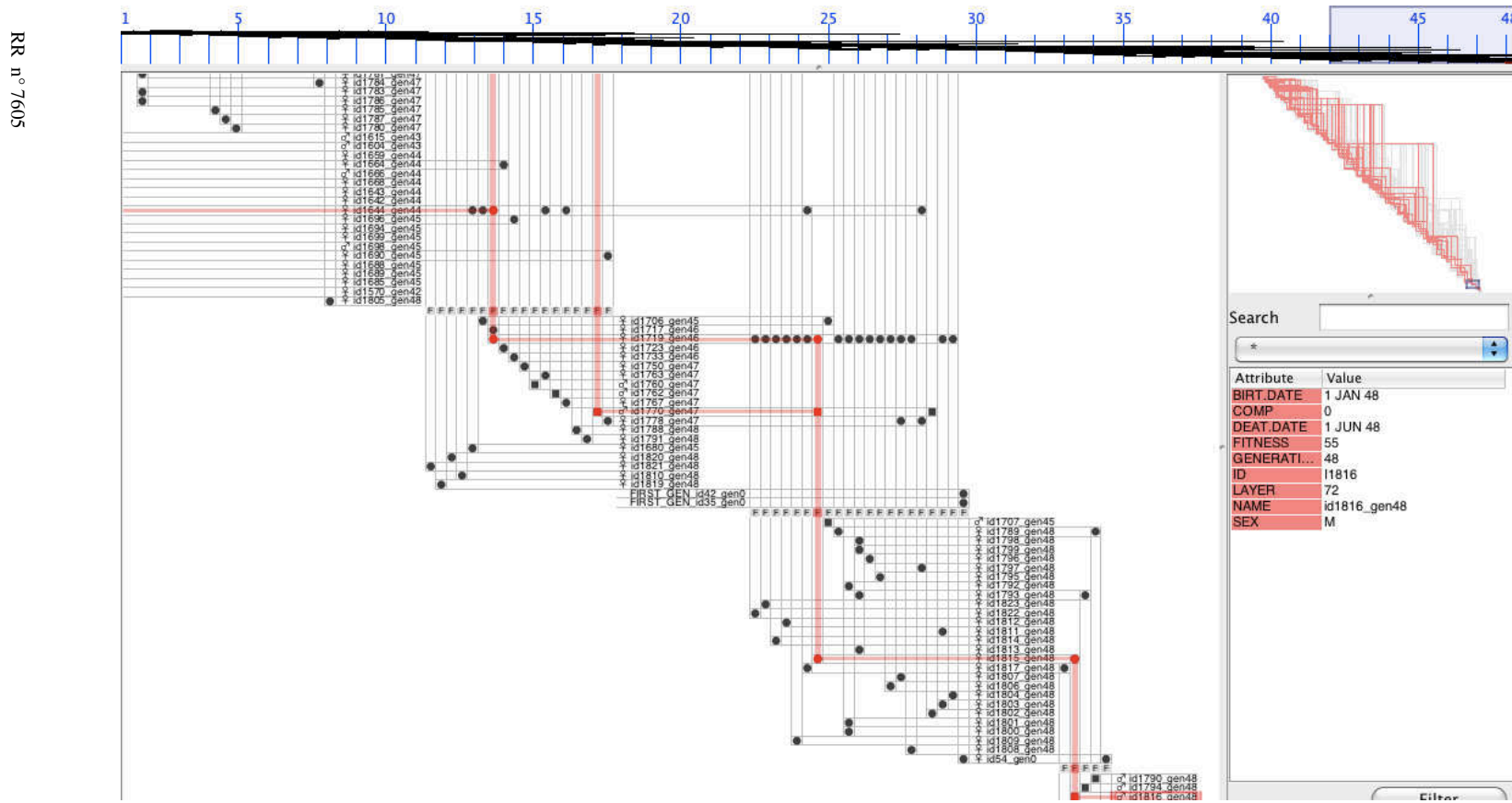
Figure 10: Rosenbrock function in dimension 10 (50 individuals during 50 generations). Zoom on the last generations and track of the ancestor of a good individual (in red)
