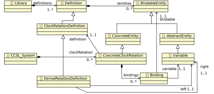
Figure 4. Simplified extendable CCSL metamodel
