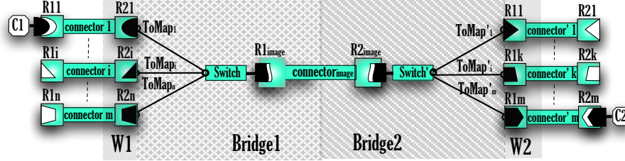
Fig. 15. Transparent interoperability
