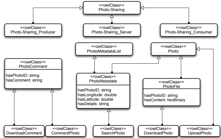
Fig. 24. Photo sharing ontology
