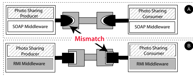
Fig. 6. Middleware mismatches
