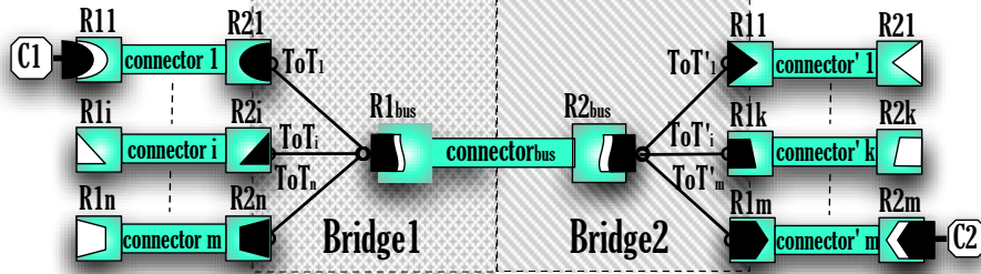
Fig. 11. Indirect bridge
