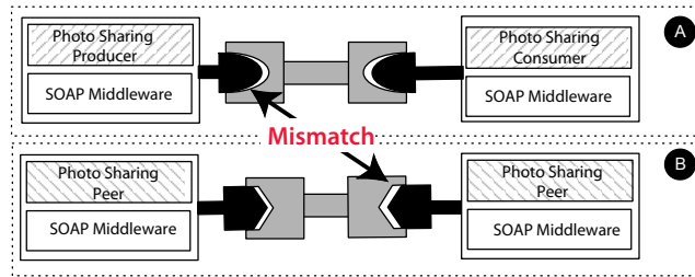
Fig. 5. Application mismatches
