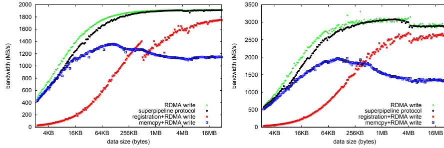
Fig. 6. Raw superpipeline protocol performance on cluster graphene (left) and infinii (right).
