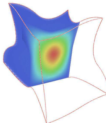
(h) solution field w.r.t optimized parameterization
