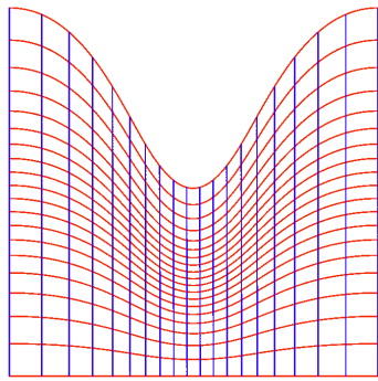
(b) initial Coons parameterization
