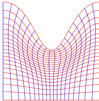
(e) optimized isoparametric net
