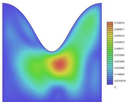
(f) simulation error w.r.t Coons parameterization
