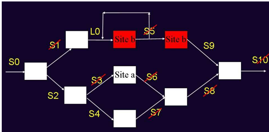
Figure 4. Asymmetric checkpoints.
