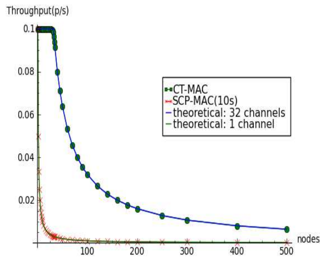
Figure 8: Throughput: CT allocation is near-optimal
