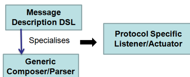
Figure 4.1: The approach for generating Listeners and Actuators
