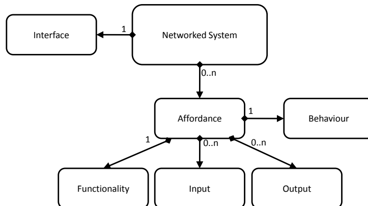
Figure 2.8: Overview of the Networked System Model
