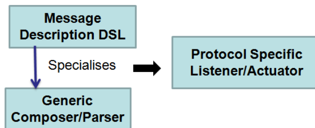
Figure 4.1: The approach for generating Listeners and Actuators
