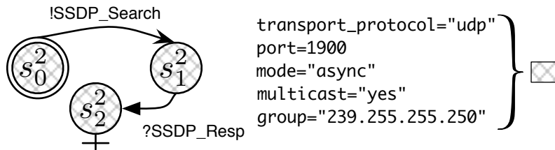
Figure 4.7: SSDP coloured LTS
