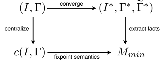
Figure 2: Link with centralized semantics
