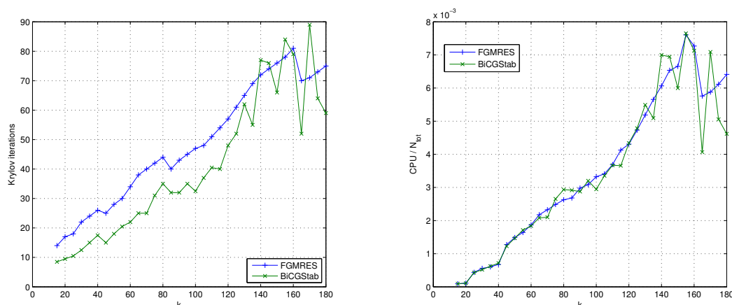
Figure 2: Left: the number of FGMRES and Bi-CGSTAB iterations as a function of the wave number k for the homogeneous Helmholtz problems. Right: the CPU time of FGMRES and Bi-CGSTAB as a function of the wave number k for the homogeneous Helmholtz problems.
