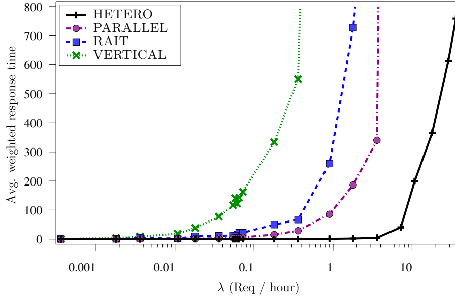
Figure 11: Impact of arrival rates on the average weighted response time (with small, medium-size and large file together, and B = 512 MB for RAIT).
