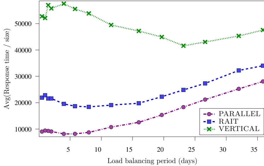
Figure 10: Impact of LOAD-BALANCER period on performance.
