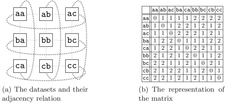
Fig. 4. Universe and highest min-entropy leakage matrix giving \epsilon -differential privacy for Example 1.
