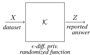
Fig. 1. Randomized function \mathcal{K}
