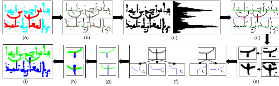
Fig. 7: Different steps of the separation of connected components.
