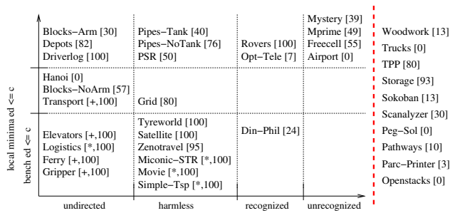
Figure 3: Overview of TorchLight domain analysis results. “*”: global analysis always succeeds; “+”: local analysis always succeeds if provided an optimal relaxed plan; mean success rates when sampling one state per domain instance.
