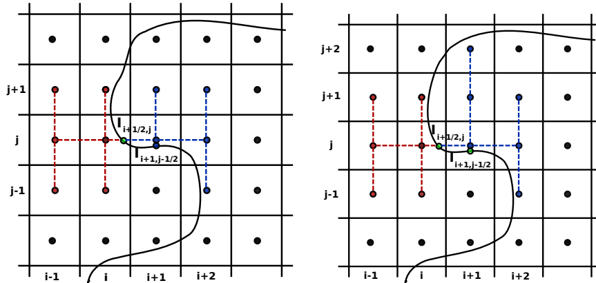
Figure 4: On left: Centered stencil: the discretization of the flux on point I_{i+1/2, j} involves intersection point I_{i+1, j-1/2} and is not numerically well-conditioned. On right: Decentered stencil: the discretization of the flux on point I_{i+1/2, j} involves now grid point (i+1, j+2) instead of intersection point I_{i+1, j-1/2}
