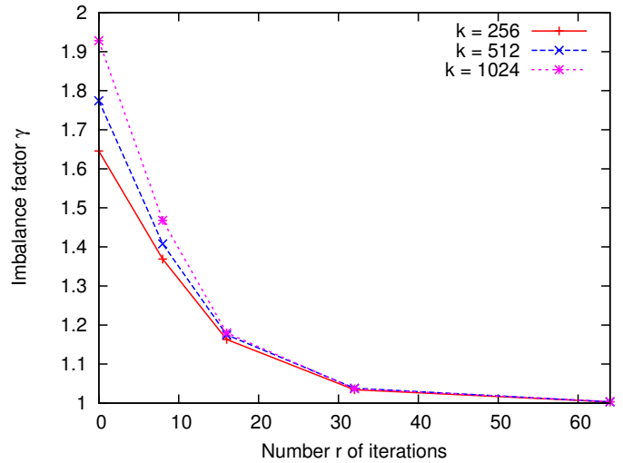
Fig. 4. Convergence speed in terms of the number r of iterations.
