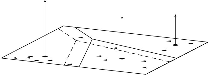
Fig. 1. Data points and centroids embedded in a 3- d example. Data points are plotted as triangles while centroids are represented as dots, with a non-null z -axis value after some iterations. Initial Voronoi region boundaries and their shifted version are respectively plotted as solid and dashed lines.
