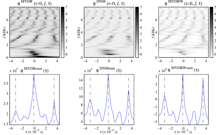
Figure 1: Local angular spectra \phi(t, f, \tau) plotted at time t = 0 (top) and pooled angular spectra \phi^{\text{sum}}(\tau) (bottom) for \phi^{\text{MVDR}} (left), \phi^{\text{DNM}} (center) and \phi^{\text{MVDRW}} (right), computed from the mixture of three female speech sources placed at 50 cm from the center of the microphone pair, with d = 15 cm and a reverberation time of 500 ms. Dash-dotted lines indicate the true TDOAs.
