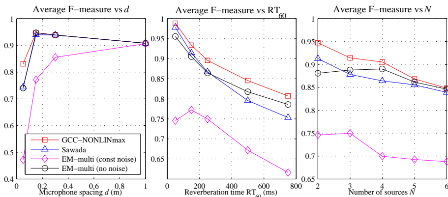
Figure 5: Clustering-based methods: average F-measure as a function of microphone spacing d (left), reverberation time RT_{60} (center), and number of sources N (right).
