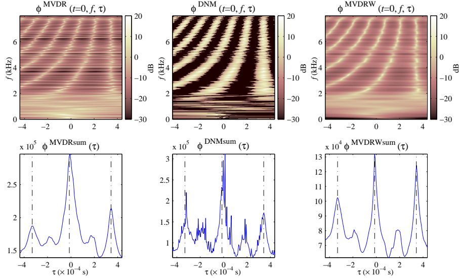
Figure 1: Local angular spectra \phi(t, f, \tau) plotted at time t = 0 (top) and pooled angular spectra \phi^{\text{sum}}(\tau) (bottom) for \phi^{\text{MVDR}} (left), \phi^{\text{DNM}} (center) and \phi^{\text{MVDRW}} (right), computed from the mixture of three female speech sources placed at 50 cm from the center of the microphone pair, with d = 15 cm and a reverberation time of 500 ms. Dash-dotted lines indicate the true TDOAs.
