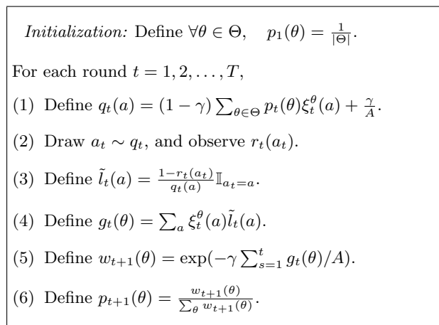
Figure 2: The Exp4 meta algorithm
