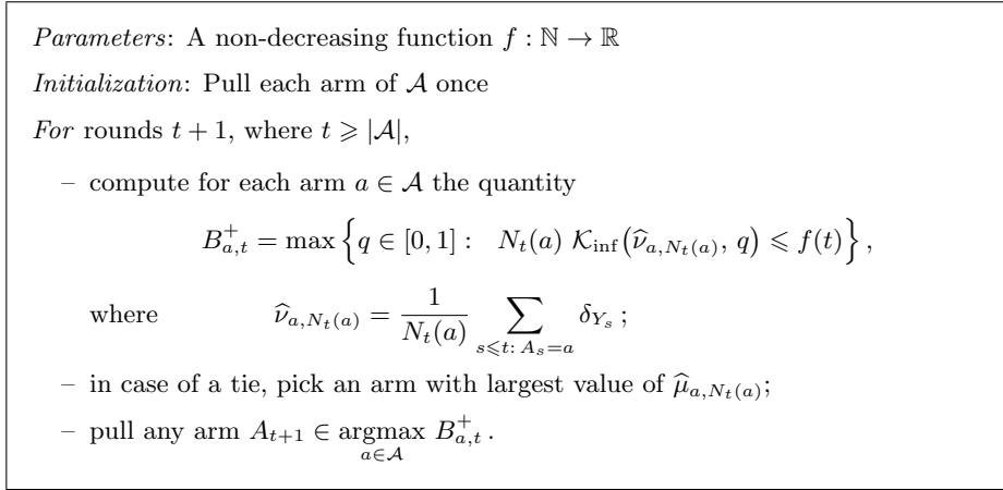
Figure 2: The strategy \mathcal{K}_{\text{inf}} .
