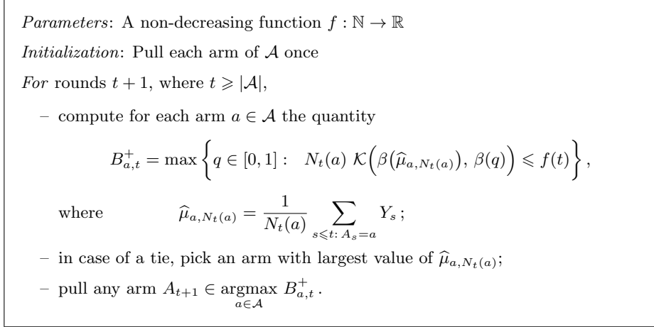
Figure 1: The \mathcal{K} -strategy.
