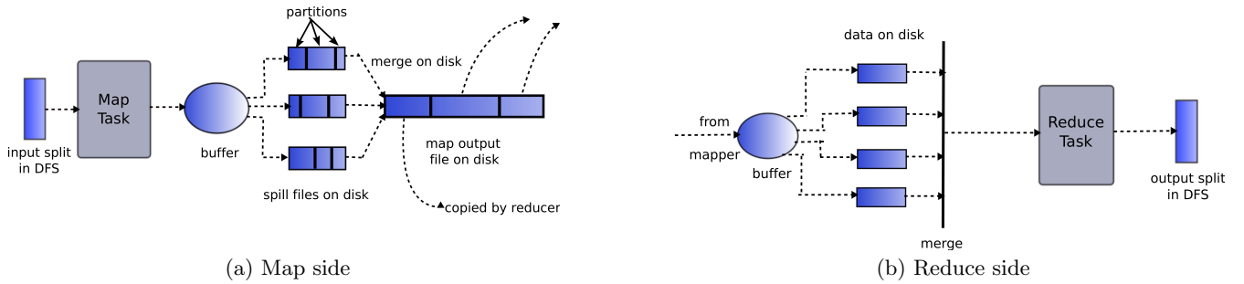
Figure 1: Intermediate data in the original Hadoop MapReduce framework
