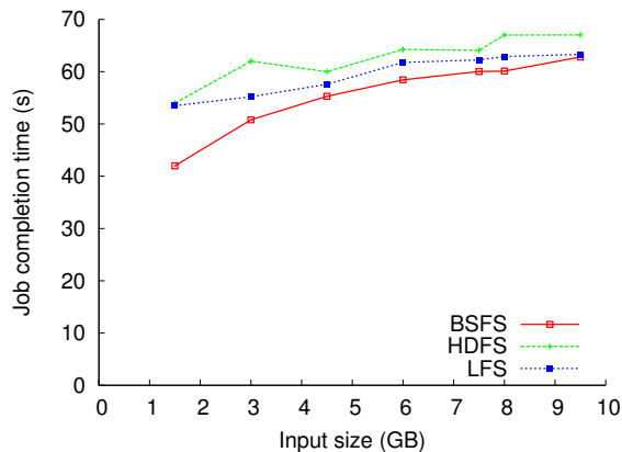
Figure 5: Distributed grep
