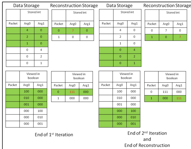
Figure 14: End of xor-ings, final state of Reconstruction phase
