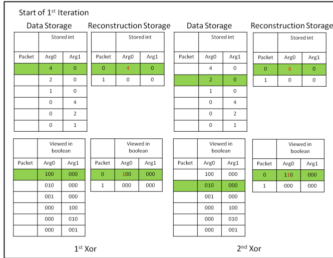
Figure 13: First xor-ings of the Reconstruction phase
