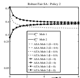
Fig. 6. Robust Policy 2 : Maximal ASA and corresponding ATA shares versus \alpha .
