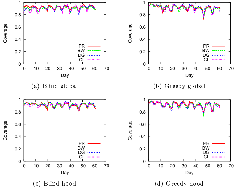
Figure 6: Coverage potential in time for all strategies ( Dartmouth data-set).
