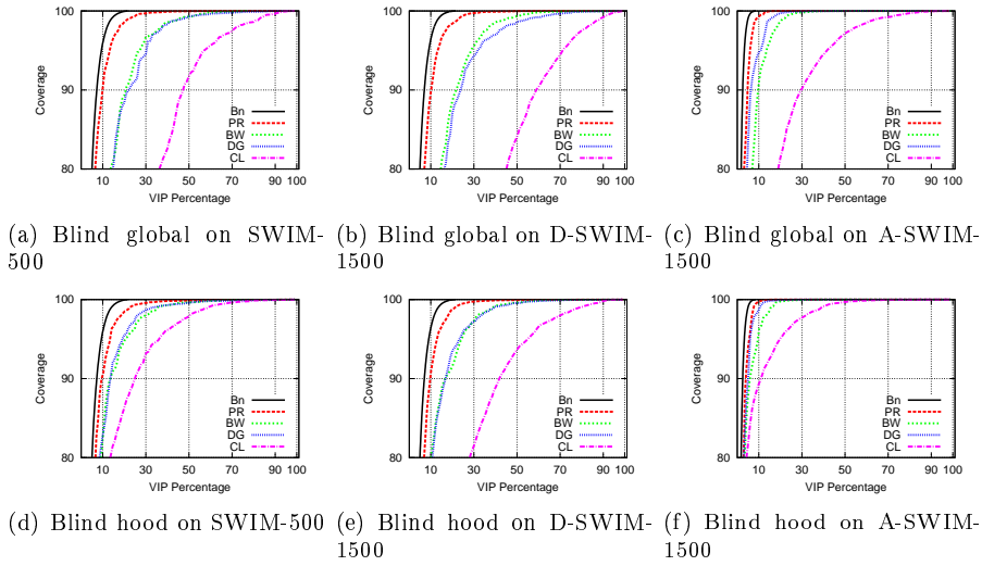
Figure 7: Performance of (a)-(c) blind global and (d)-(f) blind hood selection on SWIM. “Bn” refers to the benchmark, “PR” to the page-rank, “BW” to betweenness centrality, “DG” to degree centrality, and “CL” to closeness centrality.
