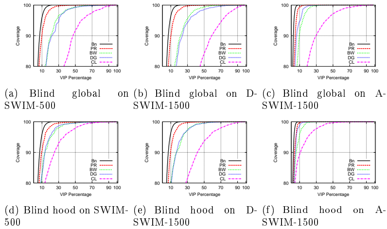
Figure 7: Performance of (a)-(c) blind global and (d)-(f) blind hood selection on SWIM. “Bn” refers to the benchmark, “PR” to the page-rank, “BW” to betweenness centrality, “DG” to degree centrality, and “CL” to closeness centrality.
