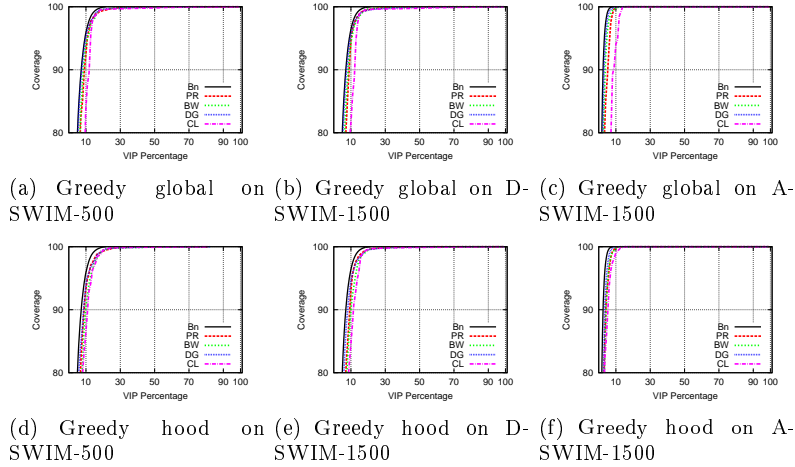
Figure 8: Performance of (a)-(c) greedy global and (d)-(f) greedy hood selection on SWIM. “Bn” refers to the benchmark, “PR” to the page-rank, “BW” to betweenness centrality, “DG” to degree centrality, and “CL” to closeness centrality.
