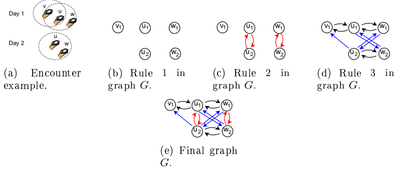
Figure 1: (a) Meeting between u , v , and w during days 1 and 2. (b)-(d) Rules for the construction of graph G . (e) Final representation of graph G .
