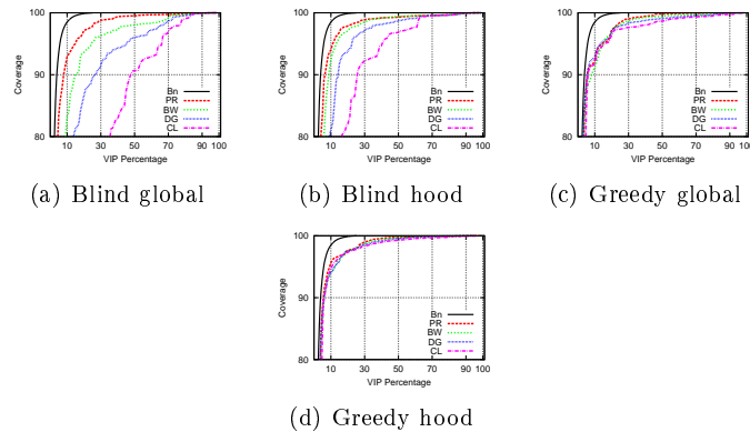
Figure 2: Performance of the selection strategies on the Dartmouth data-set. “Bn” refers to the benchmark, “PR” to the page-rank, “BW” to betweenness centrality, “DG” to degree centrality, and “CL” to closeness centrality.
