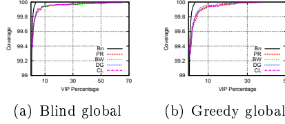
Figure 5: Performance of blind global and greedy global selection strategies on the Taxi data-set. “Bn” refers to the benchmark, “PR” to the page-rank, “BW” to betweenness centrality, “DG” to degree centrality, and “CL” to closeness centrality.
