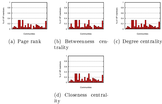
Figure 4: Distribution of VIPs per social attribute on the Dartmouth dataset with the greedy global promotion strategy. The x-axis represents different communities detected.
