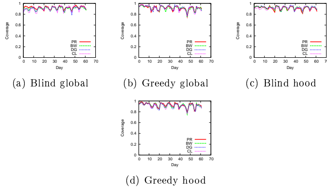
Figure 6: Coverage potential in time for all strategies ( Dartmouth data-set).
