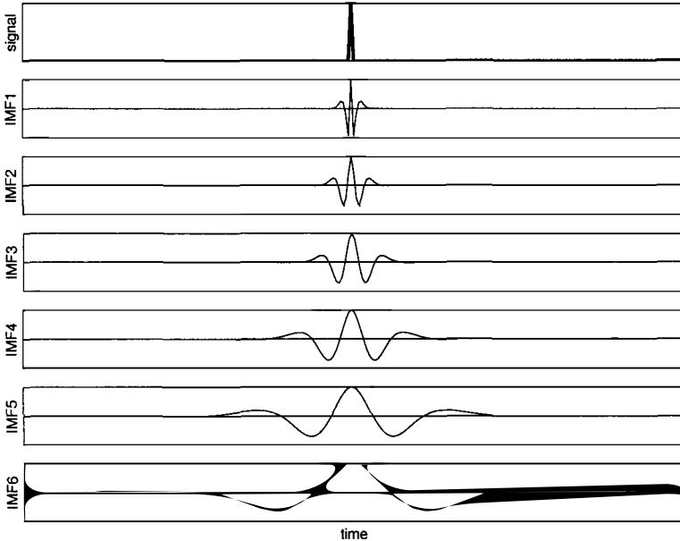
Figure 3.4: Impulse response. The EMD equivalent impulse response was obtained by averaging each IMF by using a large number of decompositions computed with a slightly noisy pulse. Here, 5 000 independent realizations from 256 data points were simulated with a signal-to-noise ratio of 34 dB. The first frame shows the average pulse and each successive frame corresponds to the ensemble average of the first six IMFs normalized in amplitude mode by mode.
