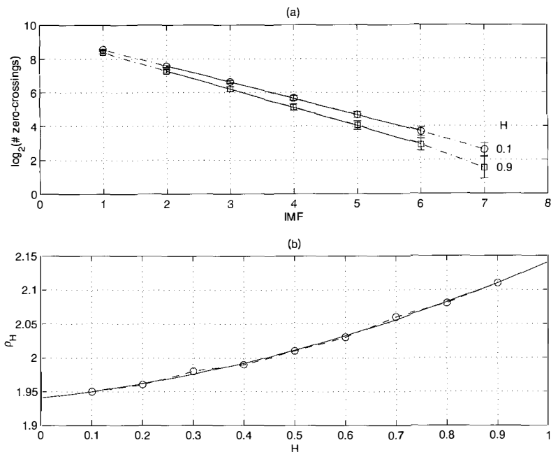
Figure 3.2: (a) IMF average number of zero-crossings z_H[k] in the case of fractional Gaussian noise. For clarity, only those curves corresponding to the extreme indices H = 0.1 (circles) and H = 0.9 (squares) have been plotted in the diagram; the remaining cases ( H = 0.2, 0.3, \dots, 0.8 ) lead to regularly intertwined similar curves. The superimposed solid lines correspond to linear fits within the IMF range k = 2 to 6. (b) Corresponding decrease rate of zero-crossings (circles and dashed line), with the least-squares quadratic fit given by (3.4) superimposed as a solid line. (Originally published in Int. J. Wavelets Multiresolut. Inform. Process. , 2 , 477–496, ©2004 World Scientific.)
