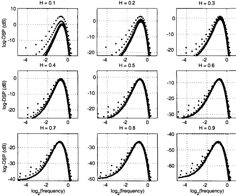
Figure 3.3: Renormalized IMF spectra in the case of fractional Gaussian noise. For each value of H , the band-pass IMFs ( k = 2 to 6 ) of Figure 3.1 are plotted according to the renormalization given by (3.5) with \alpha = 2H - 1 , and the values of \rho_H are given in Fig. 3.2b. (Originally published in Int. J. Wavelets Multiresolut. Inform. Process. , 2 , 477–496, ©2004 World Scientific.)
