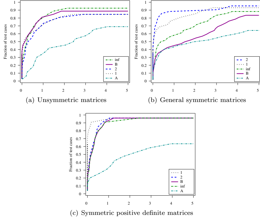
Figure 1: Performance profiles for the condition number estimates for unsymmetric matrices 1(a), general symmetric matrices 1(b), and symmetric positive definite matrices 1(c). A marks the condition number estimate of the original matrix; B marks that of Bunch’s algorithm; inf , 1 , and 2 mark that of the proposed algorithm with \infty -, 1-, and 2-norms, SK-inf marks that of Sinkhorn–Knopp with \infty -norm and rdiag marks that of the reciprocal square root of the diagonal scaling for the symmetric positive definite matrices.
