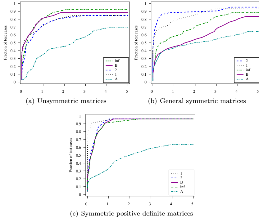
Figure 1: Performance profiles for the condition number estimates for unsymmetric matrices 1(a), general symmetric matrices 1(b), and symmetric positive definite matrices 1(c). A marks the condition number estimate of the original matrix; B marks that of Bunch’s algorithm; inf , 1 , and 2 mark that of the proposed algorithm with \infty -, 1-, and 2-norms, SK-inf marks that of Sinkhorn–Knopp with \infty -norm and rdiag marks that of the reciprocal square root of the diagonal scaling for the symmetric positive definite matrices.
