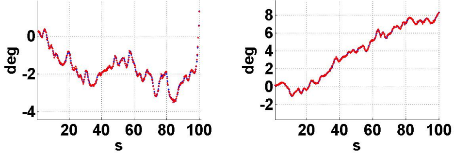
Figure 7: Roll (left) and pitch (right) angles during the simulated experiment. The blue dots are the ground truth and the red dots the estimated values.
