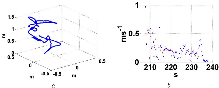
Figure 11: In a : the trajectory (ground truth) in the 3D real data set during the time interval [200, 240]s. In b : the vehicle speed in the real 3D experiment. Blue dots are the ground truth and red dots the estimated values.
